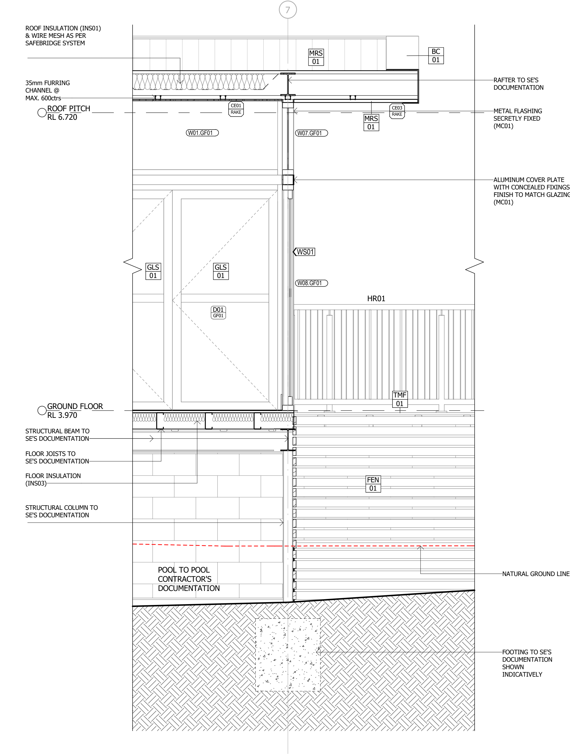
2 DETAIL SECTION 4 A3001 1 : 20
