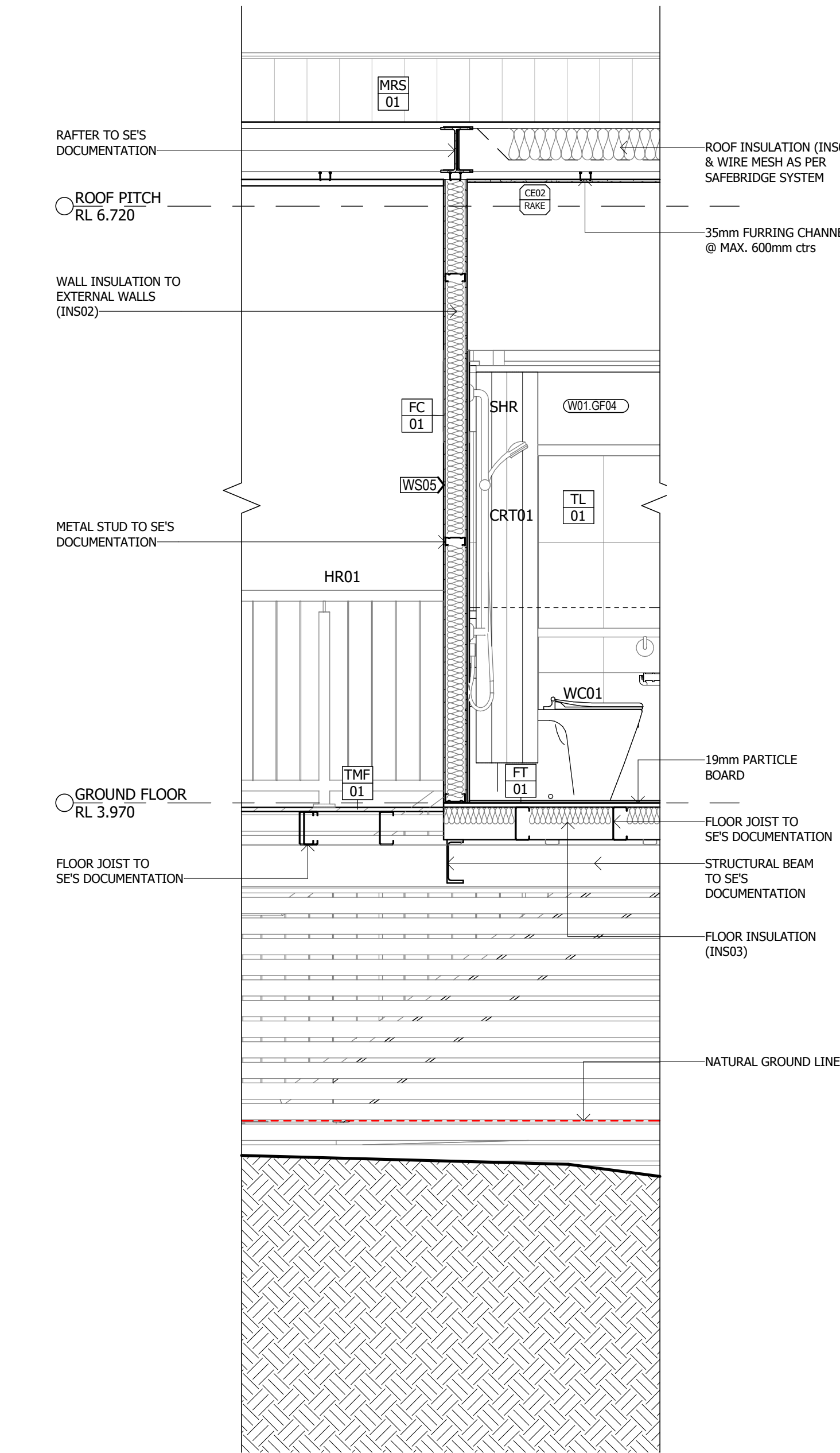
1 DETAIL SECTION 3 A3001 1 : 20
